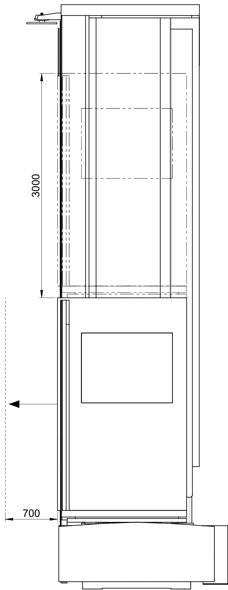
CORSE PEDANA OPERATORE OPERATOR PLATFORM'S STROKES
